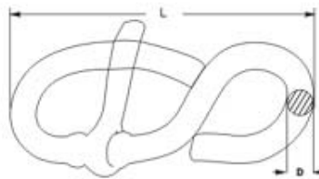
Rope Shortening 8-Shaped With Tongue Zinc Plated
